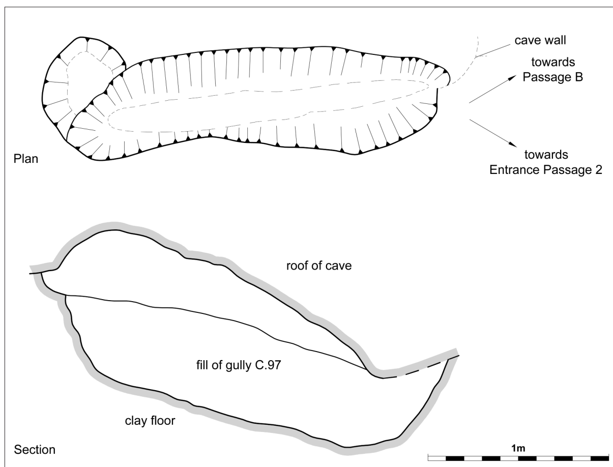
Fig. 16—Plan and section of gully cut (C.30) and gully fill (C.97) in the Main Chamber (Sq.A7).
